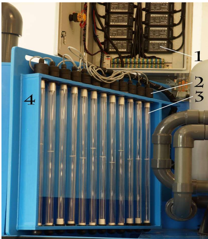
Pict. 2: 12 x UV-C lamps with 20 watts each
